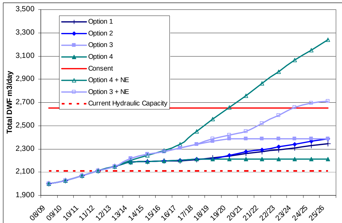
Figure 8-25 Worst Case Scenario (with constant occupancy rates) Total DWF predictions for Stansted Mountfitchet WwTW by Option, with and without northeast Elsenham (NE)
