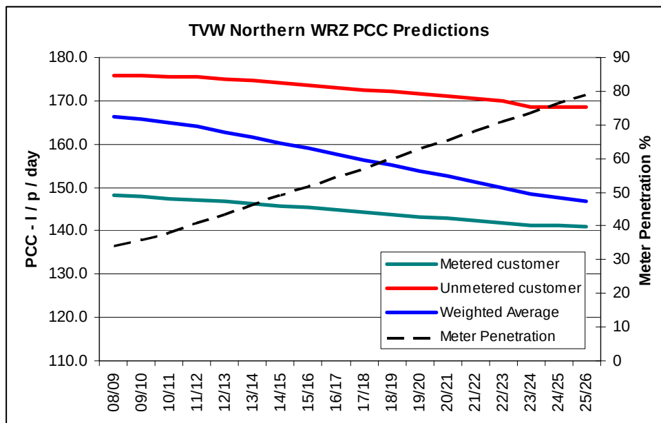
Figure 4-7 Average PCC predictions for existing population, weighted by meter penetration, as per TVW [now VW] WRMP 2009
