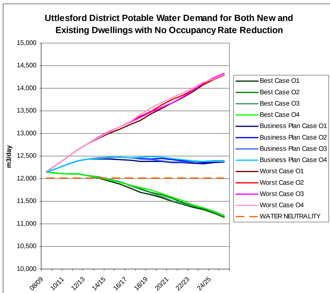
Figure 6-17 Prediction of Total Demand from all Dwellings with no decrease in Occupancy
